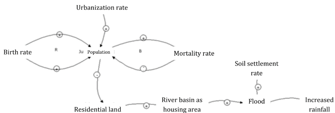
Fig. 1. Casual loop diagram (CLD)
