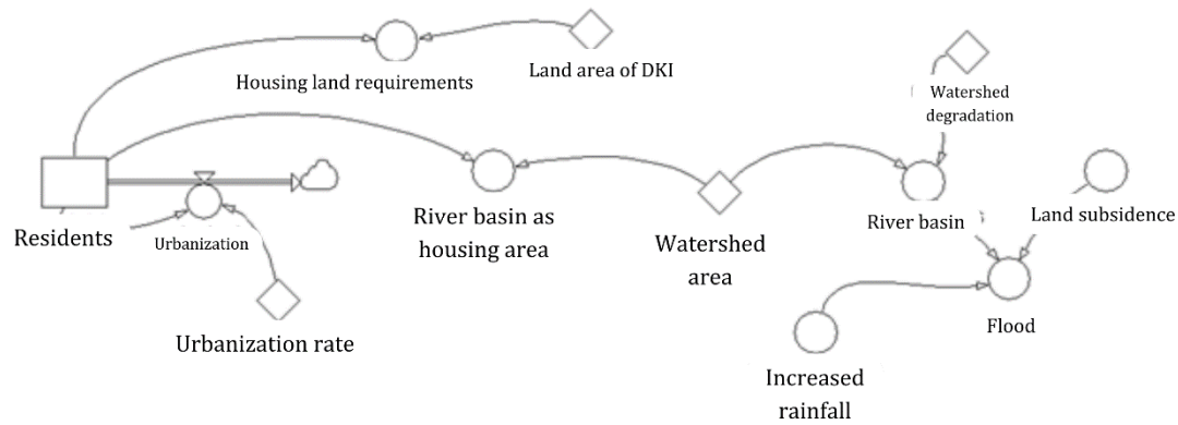
Fig. 2. Flowchart of stock flow diagram of flood events in Jakarta
